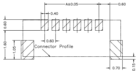
RECOMMENDED PCB LAYOUT DEFAULT TOL:±0.05
