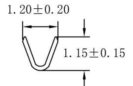
b-b section
