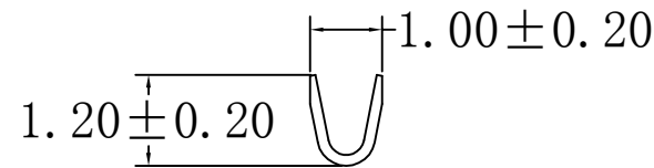
SECTION B-B
